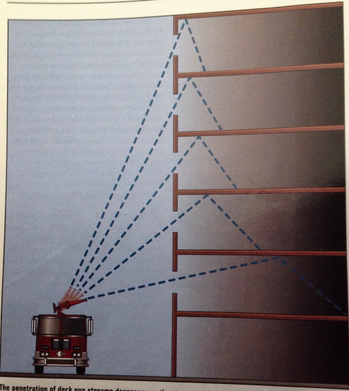
The penetration of deck gun streams decreases as the stream angles increase. (Based on an illustration from Firefighting Principles & Practices, Second Edition , by William E. Clark (Fire Engineering Books & Videos, 1991).)
